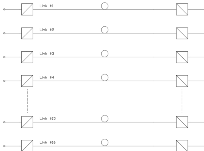
FCLS1161: 16x Single Link Schematic
