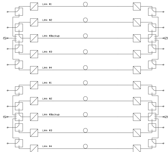
FCLR1241: 2x4+1 Link Schematic
